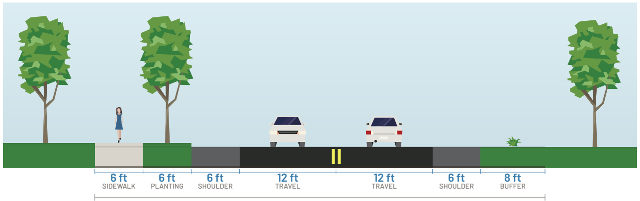
ILLUSTRATIVE SECTION · CARTWAY &amp; R.O.W. PER MAINE DOT
