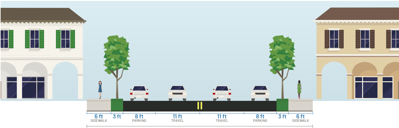
RIGHT-OF-WAY 50-62 ft range · shown at 56 ft
